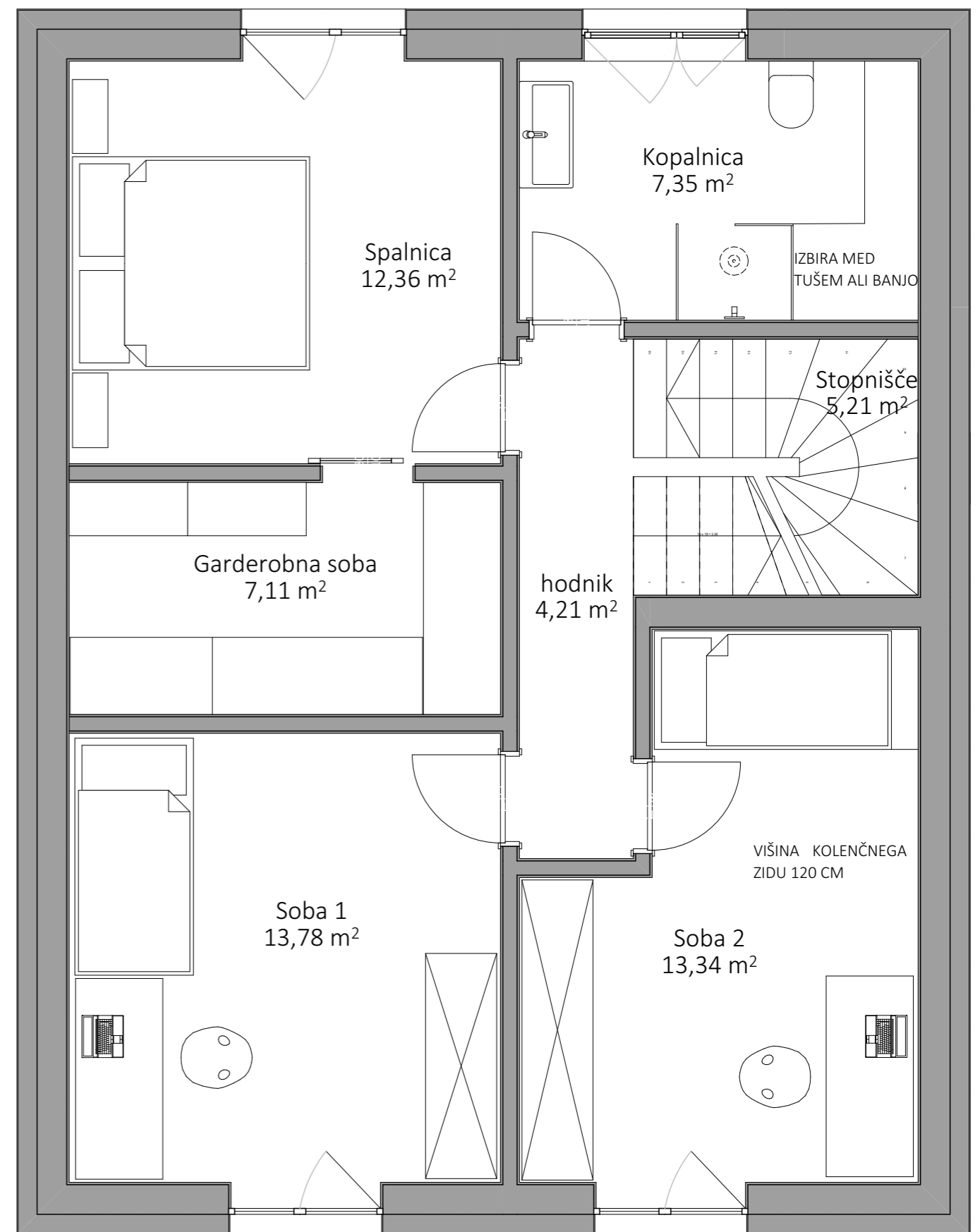
MANSARDA
